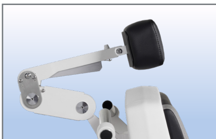
Single-handed headrest with special locking indicator
